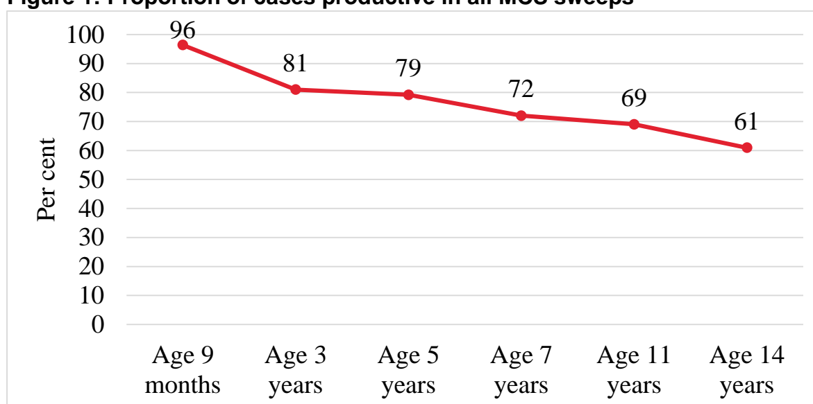
Figure 1: Proportion of cases productive in all MCS sweeps
