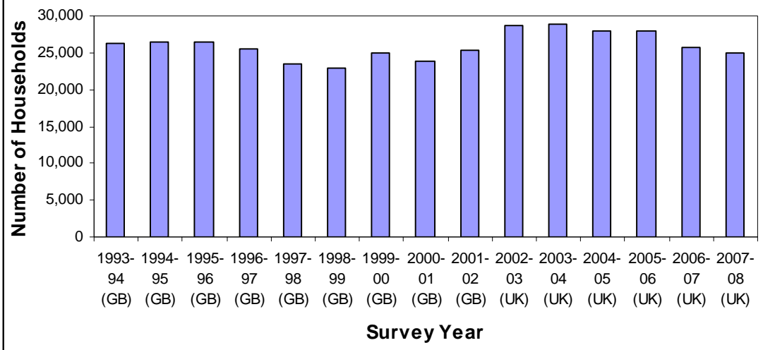
Figure 5: FRS Achieved Sample Size
